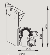
Under-roof installation
